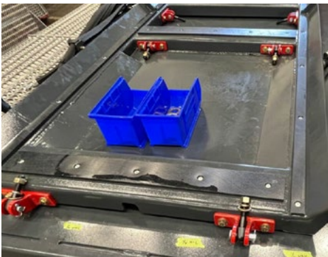
Integrated drill mounts and drip tray
